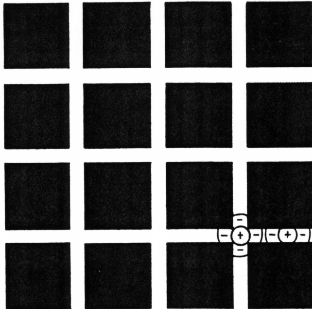
Fig. 6.8. The Hermann grid, with 2 ganglion cell receptive fields projected on it.
