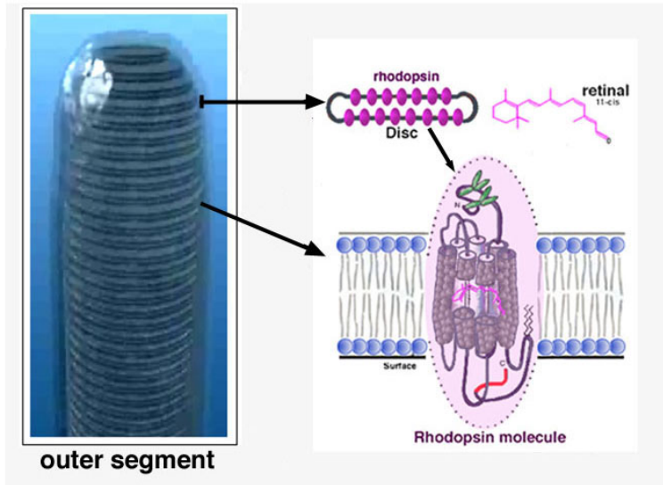
Fig. 3. Schematic diagram of Rhodopsin in the outer segment discs. When the outer segments are magnified further, stacked membrane disks are visible inside. The disks are studded with thousands of rhodopsin complexes. Each rhodopsin consists of a membrane-traversing protein with a retinal molecule embedded in its core.
